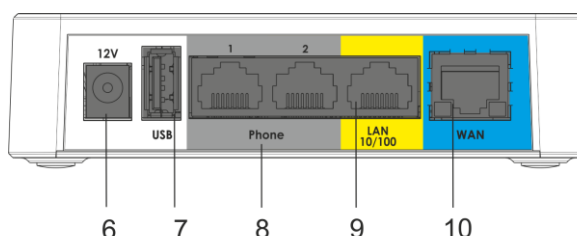
Figure 5 – TAU-2M.IP rear panel appearance
